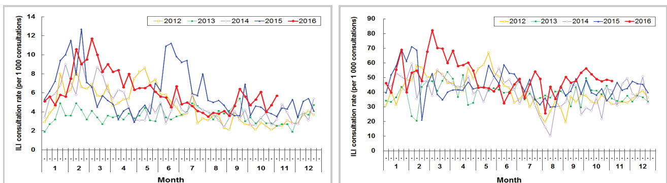
Figure 1 ILI consultation rate at sentinel GOPCs (left) and private doctors (right), 2012-16
